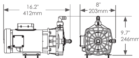
Booster Pump
